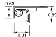
Cross Section of 16 gauge Body & Door
