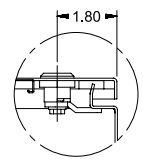
DETAIL C QUARTER TURN LOCK
