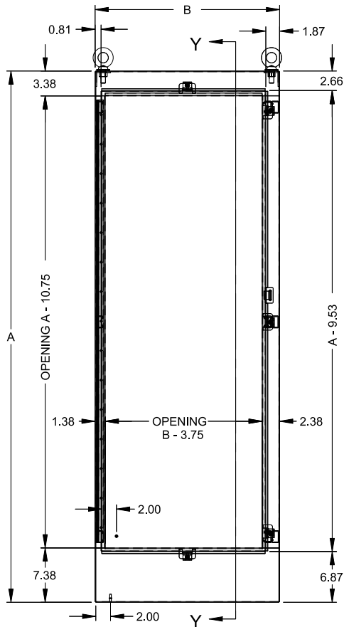
Front View
