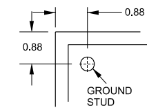
Ground Stud Location 1414N4ALA Only
