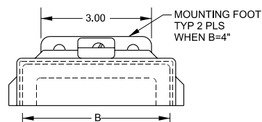
Mounting Foot Detail
